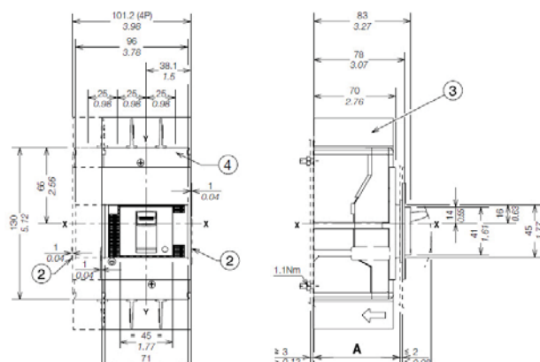
① Insulating plate obligatory ② Overall dimension of optional wiring ducts ③ 25mm insulating barriers between phases (compulsory) provided ④ Front carter obligatory for through door of the panel \leq 25\text{mm}/0.98''
